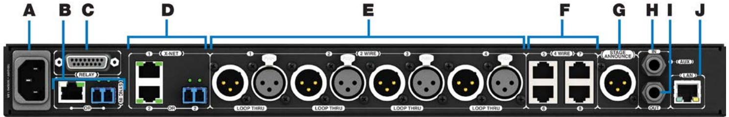
Figure 29: XCU-44 Back View
