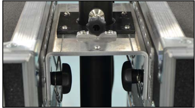
Figure 9: Top Mounting Plate with Mast Secured
