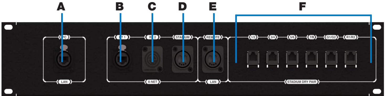
Figure 101: Wireless Press Box Rear Patch Panel
