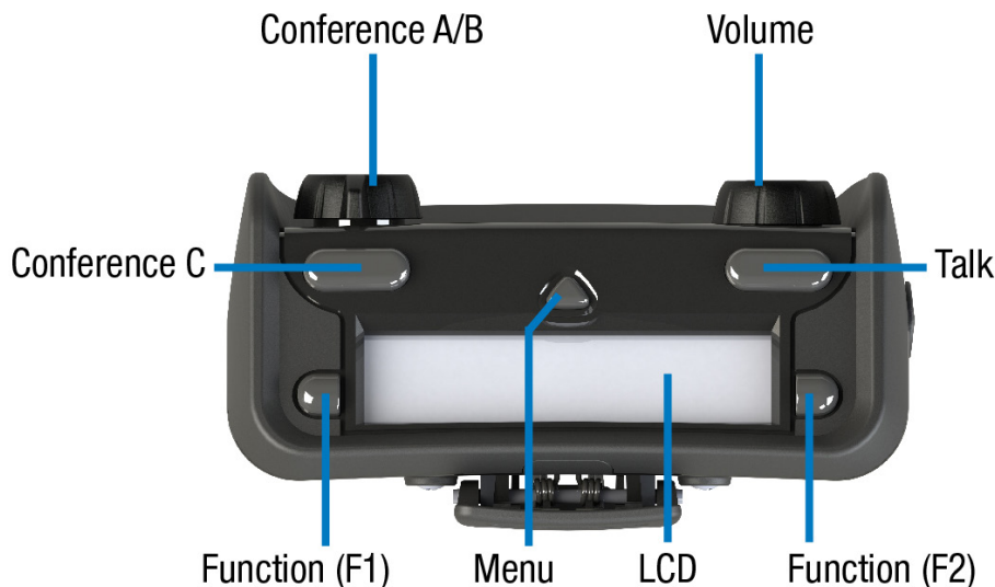
Figure 34: XRP-13 Top View
