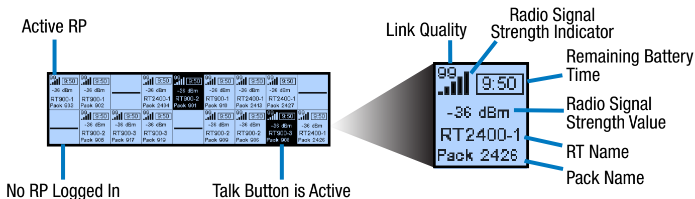
Figure 31: Control Unit Secondary Operating Screen
