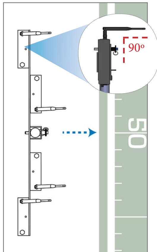
Figure 79: Top View of RT Bracket and Antenna Direction
