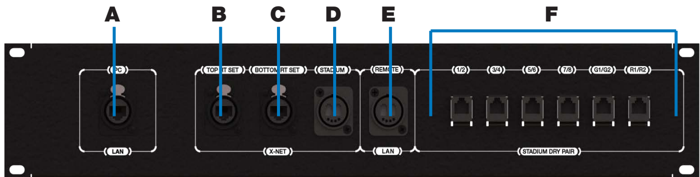
Figure 27: Sideline Wireless Trunk Rear Patch Panel
