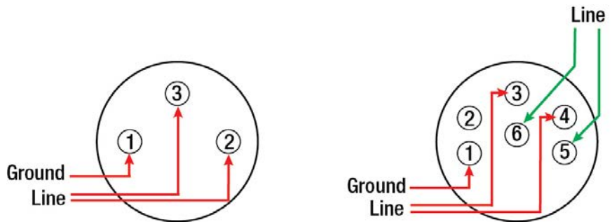
Figure 96: XLR Terminations
