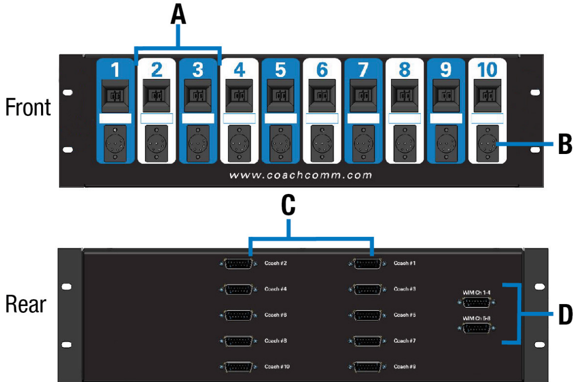
Figure 26: WAM 10 Overview
