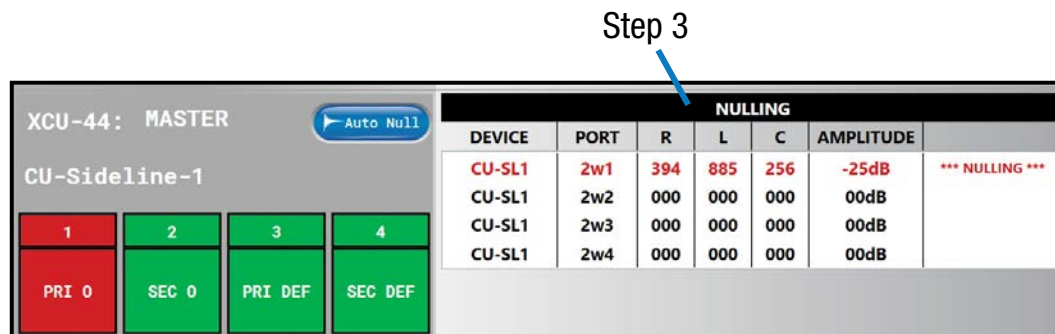
Figure 85: X-Ware Auto-Null In Progress
