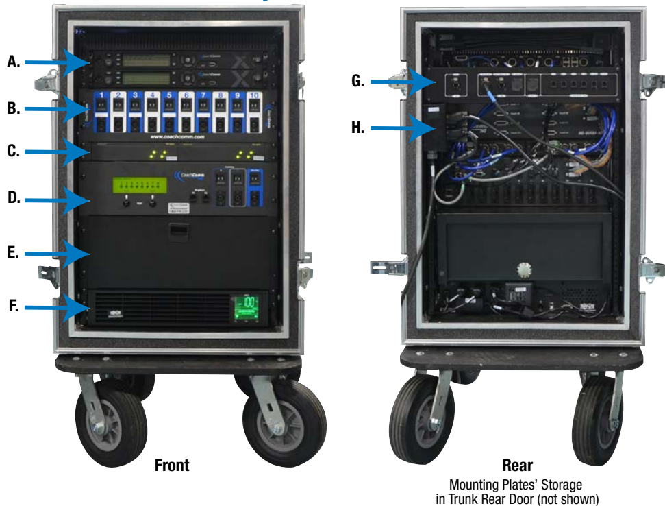
Figure 15: X-System Wireless Trunk
