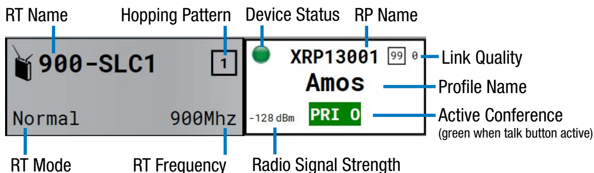
Figure 60: Radio Transceiver View Detail
