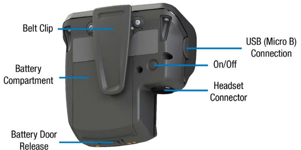
Figure 35: Radio Pack Rear View
