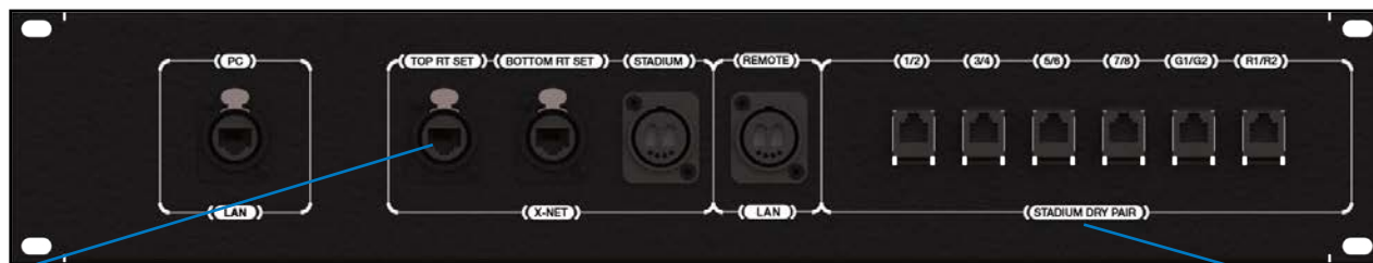
Figure 10: Sideline Wireless Trunk's rear patch panel
