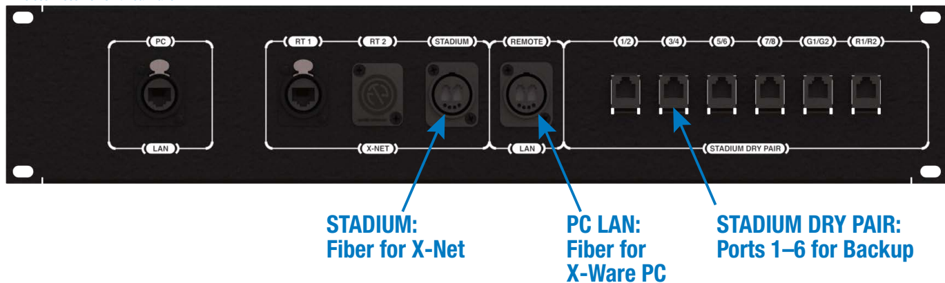
Wireless Press Box Unit Rear Panel
