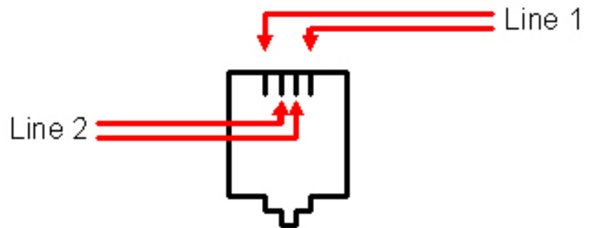
Figure 97: RJ-14 Wiring
