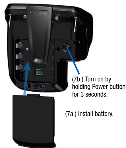
Figure 14: Radio Pack
