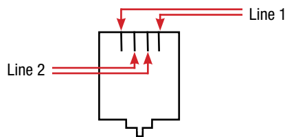
Figure 1: RJ-14 Wiring
