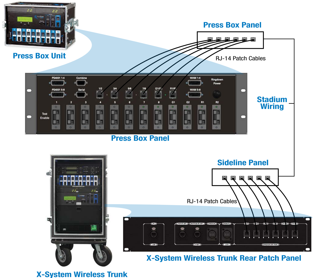
Figure 5: Sideline to Wired Press Box Unit (System Diagram)
