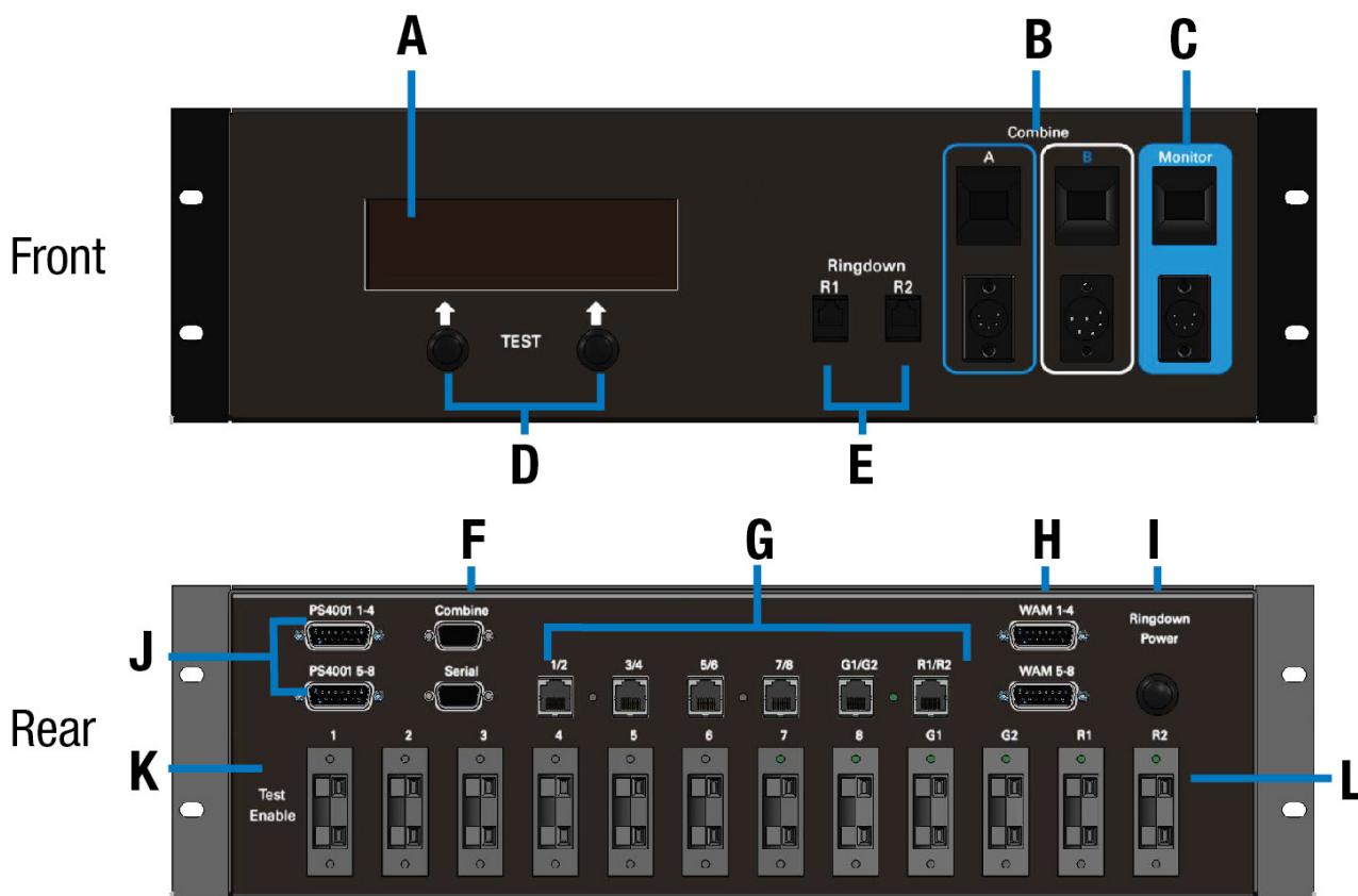
Figure 21: WIM 8 Overview
