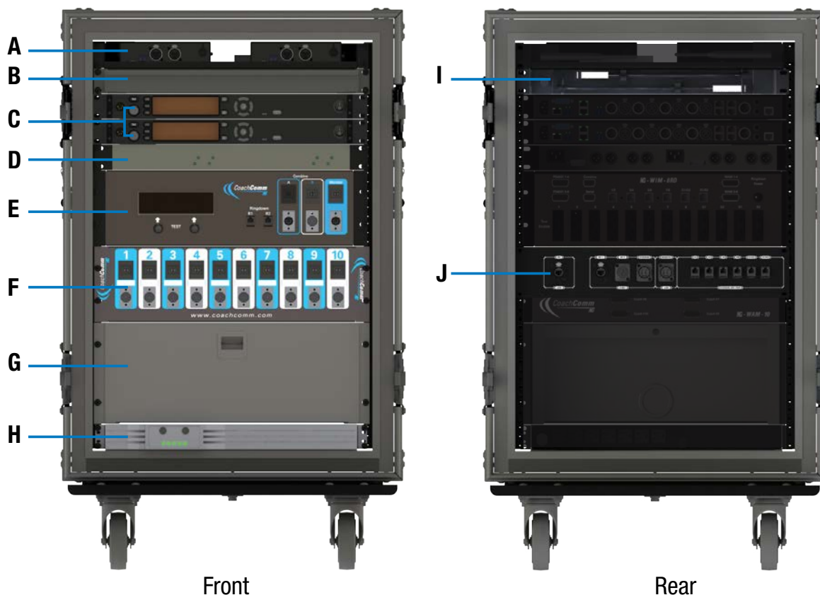
Figure 100: Wireless Press Box Unit Front View
