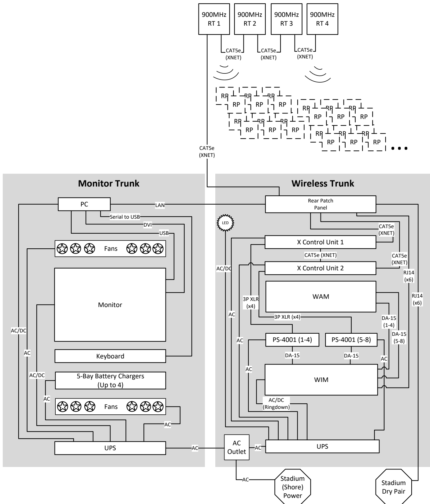
Figure 7: Sideline Trunks Block Diagram
