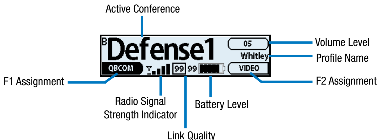
Figure 36: RP-44 Home Operating Screen
